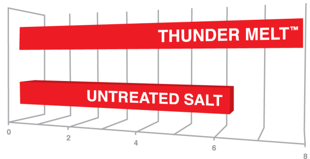
Ice melting comparisons measured in milliliters using the testing method set up by the SHRP, Strategic Highway Research Program, H-205.1. Ice melters were tested at 15°F for 20 minutes.
