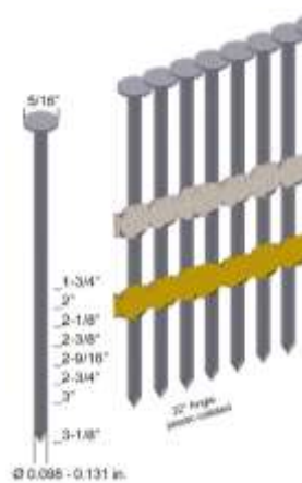
22° Plastic
