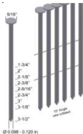
15° Wire Coil
