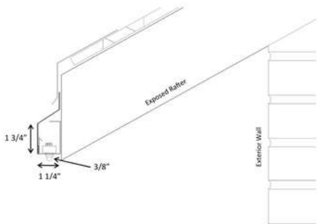
Rafter Board Installation
