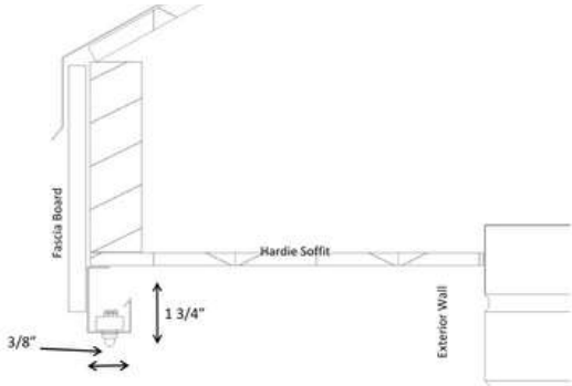
Fascia Board Installation
