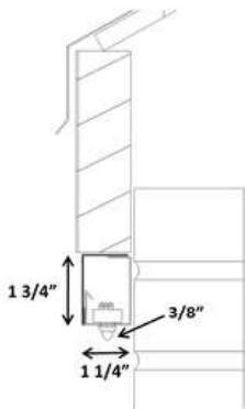
For Flush Board Installation
